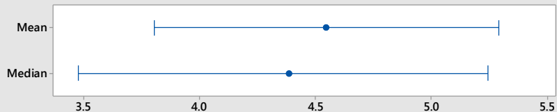
95% Confidence Intervals
